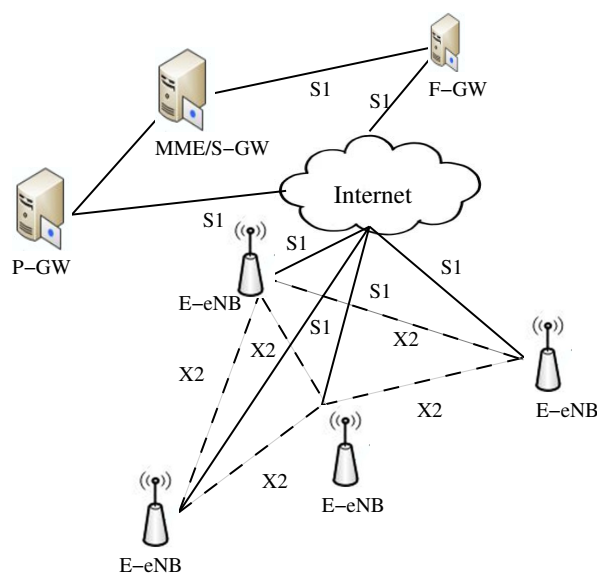
Fig. 1. Architecture of Enterprise LTE Femtocell Network
