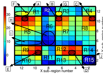
Fig. 5. DSINR (in dB) for CKM Placement of Femto
