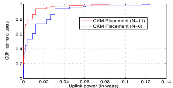
Fig. 1. CDF of UE uplink power.
