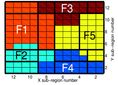
Fig. 6. Femto sub-region association for MFUTP placement
