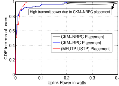
Fig. 11. Uplink Power interms of users
