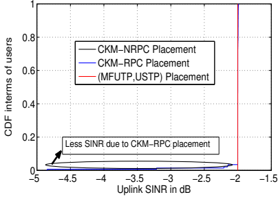
Fig. 10. Uplink SINR (in dB) interms of users
