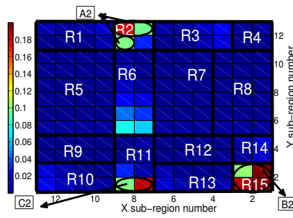
Fig. 8. Uplink power (in Watts) for CKM-RPC Placement of Femto.
