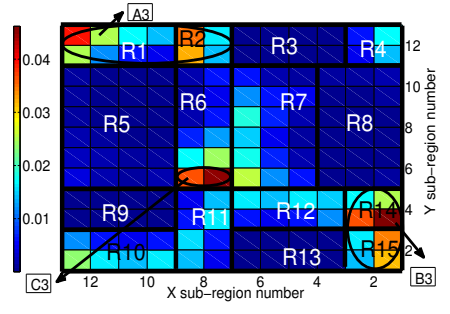
Fig. 9. Uplink Power (in Watts) for (MFUTP, USTP) Placement of Femto.
