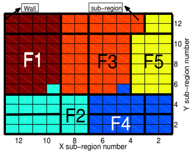
Fig. 4. Femto sub-region association for CKM Placement
