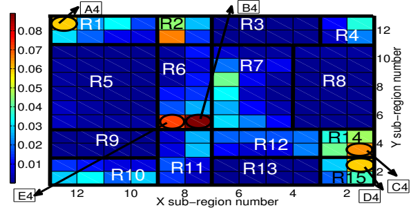
Fig. 13. Variation of Uplink Power (in Watts) based on SINR_{R_{Th}} in (MFUTP, USTP) placement
