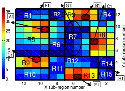
Fig. 7. DSINR (in dB) for MFUTP Placement of Femto
