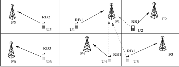
Fig. 3. Uplink Interference Scenario in Indoor Building
