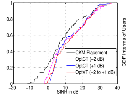
Fig. 7. SINR variation inside the building.
